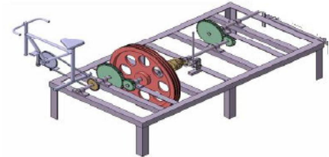
Figure 3: Bicycle mechanism with flywheel as energy unit with mechanical power transmission from input to the output by
