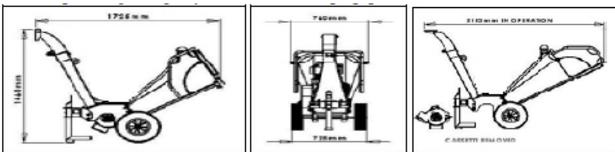
Figure 2: Main proposed process unit of wood chipper cutter machine showing the inlet and outlet manifold from different views.
