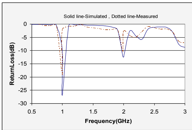
Figure 2 Variation of return loss with frequency for base shape.
