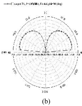
Figure 6 Radiation pattern at f=1.95\text{GHz} (a) E-total, \phi=0(\text{deg}) (b) E-total, \phi=90(\text{deg})
