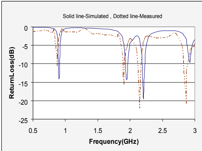
Figure 4 Variation of return loss with frequency for first iteration.
